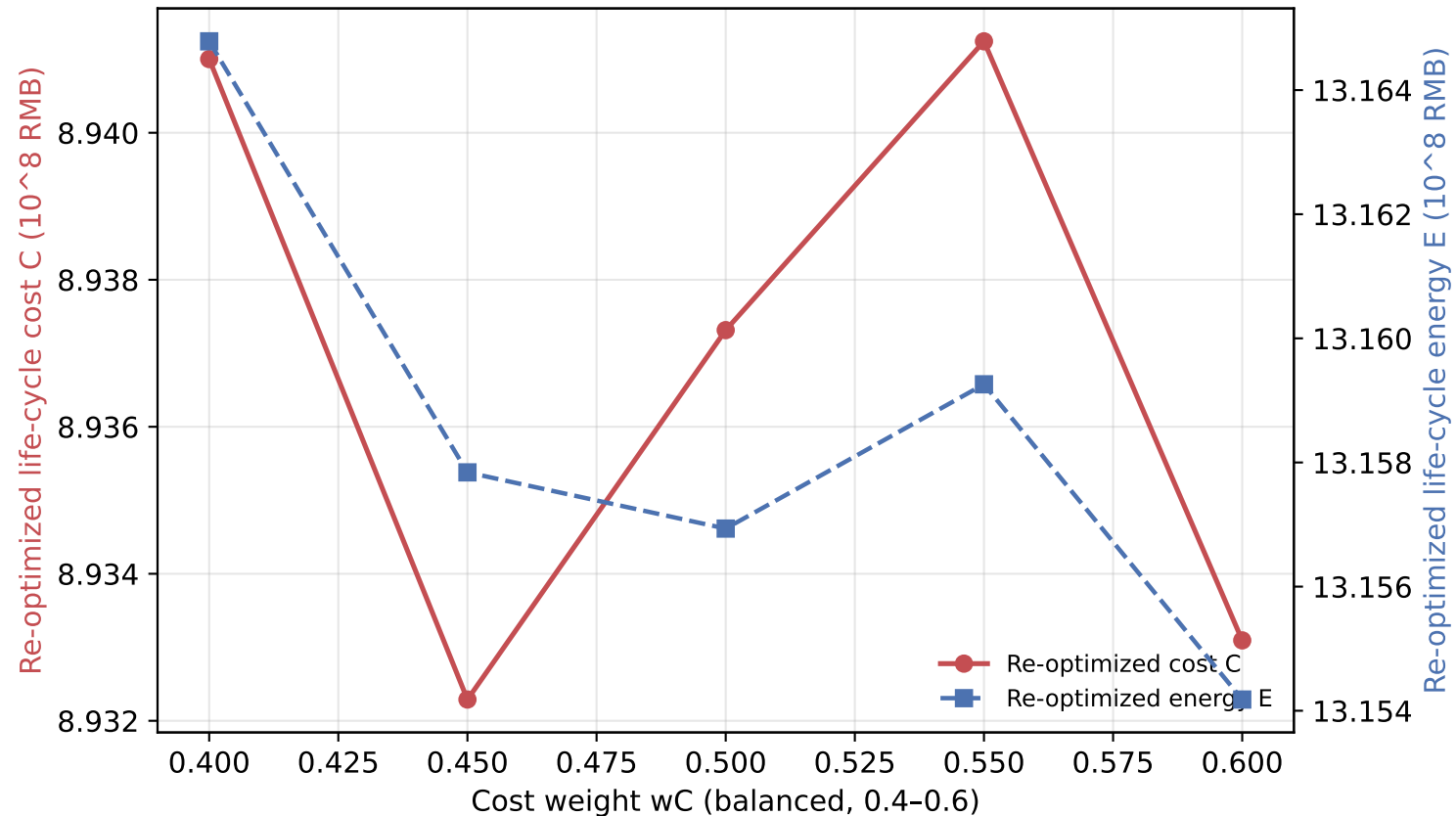
Fig. D8 Re-optimized cost & energy vs weight (balanced, wC & wE each 0.4–0.6)
