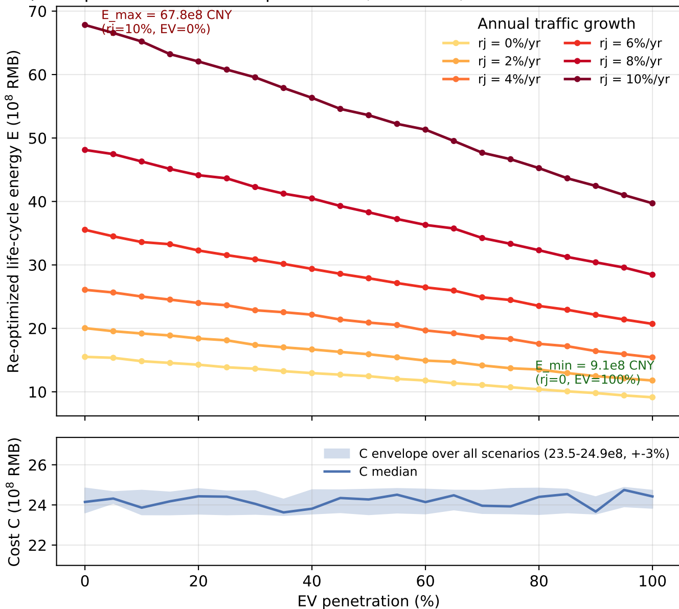
Fig. D1b Traffic growth x EV penetration: E fans out, C stays flat (each point = one full re-optimization, w_1=0.65 ; all 126 scenarios feasible)
