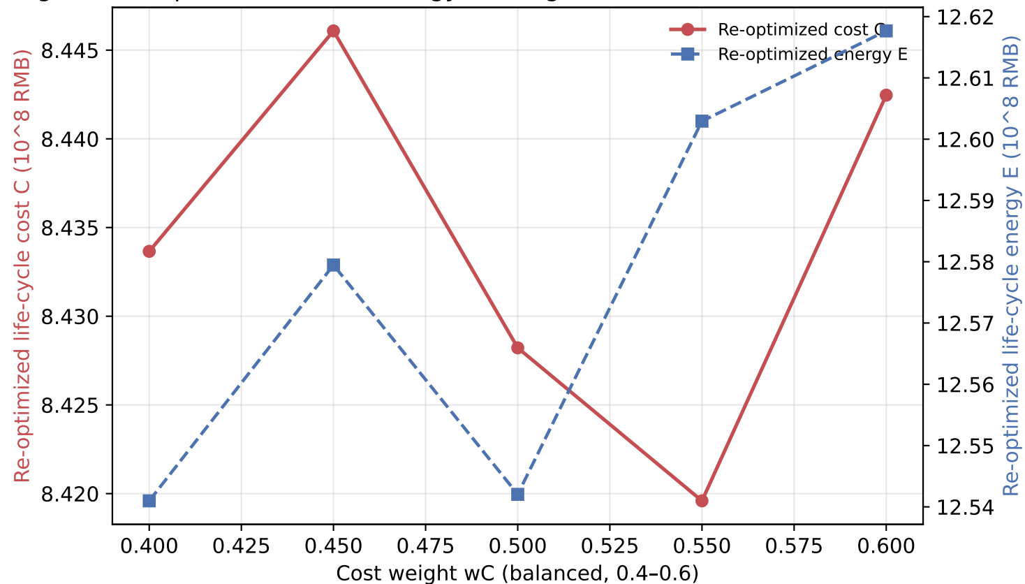
Fig. D8 Re-optimized cost & energy vs weight (balanced, wC & wE each 0.4–0.6)
