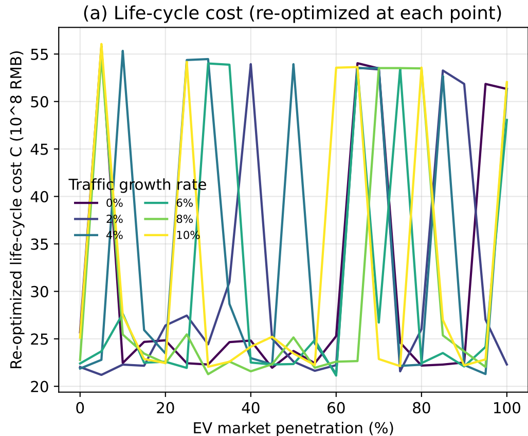
Fig. D1 Re-optimized cost and energy vs traffic growth rate and EV penetration
