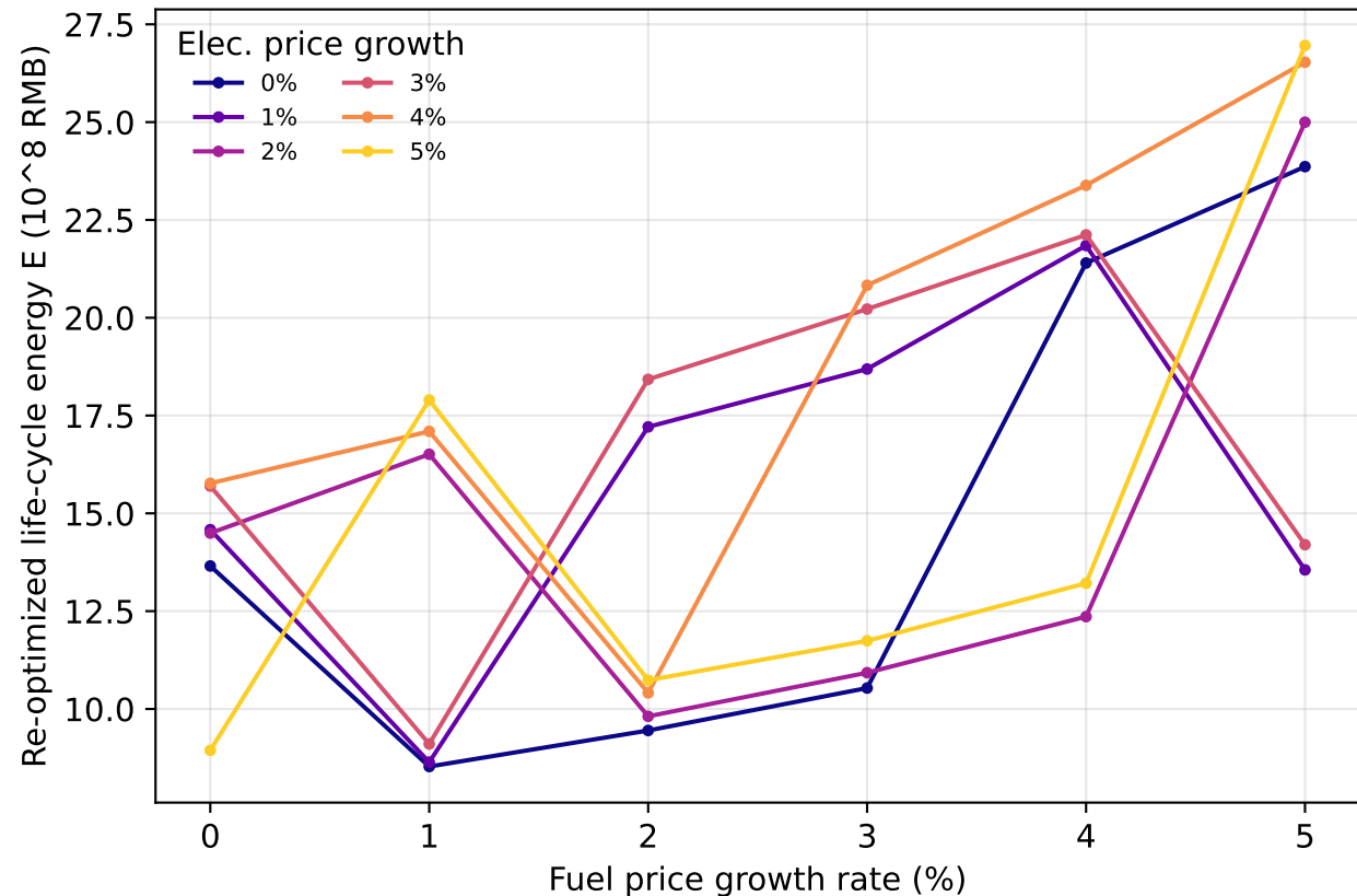
Fig. D2 Re-optimized energy vs fuel and electricity price growth
