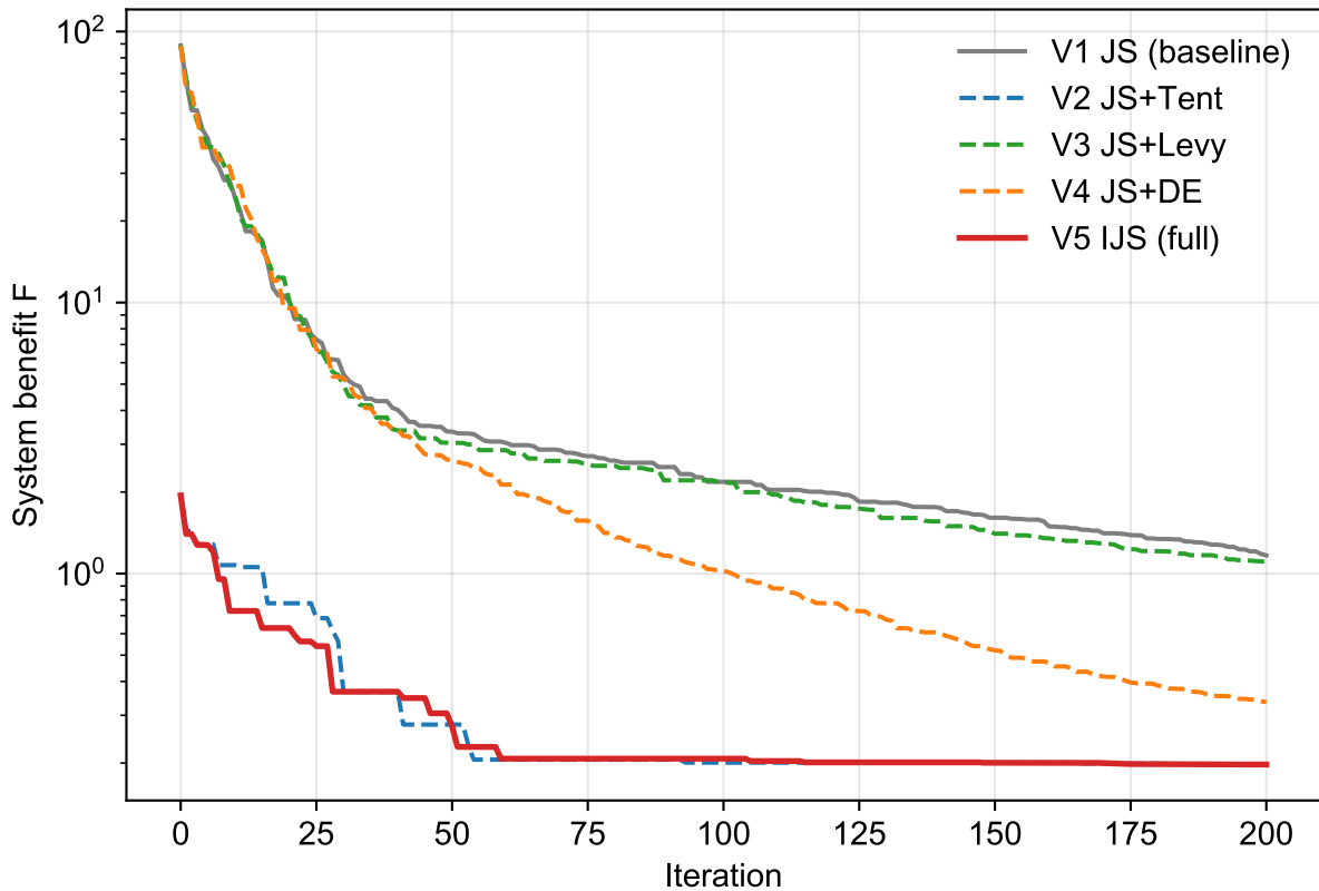
Fig. A1 Convergence curves of the five ablation variants (first 200 generations)
