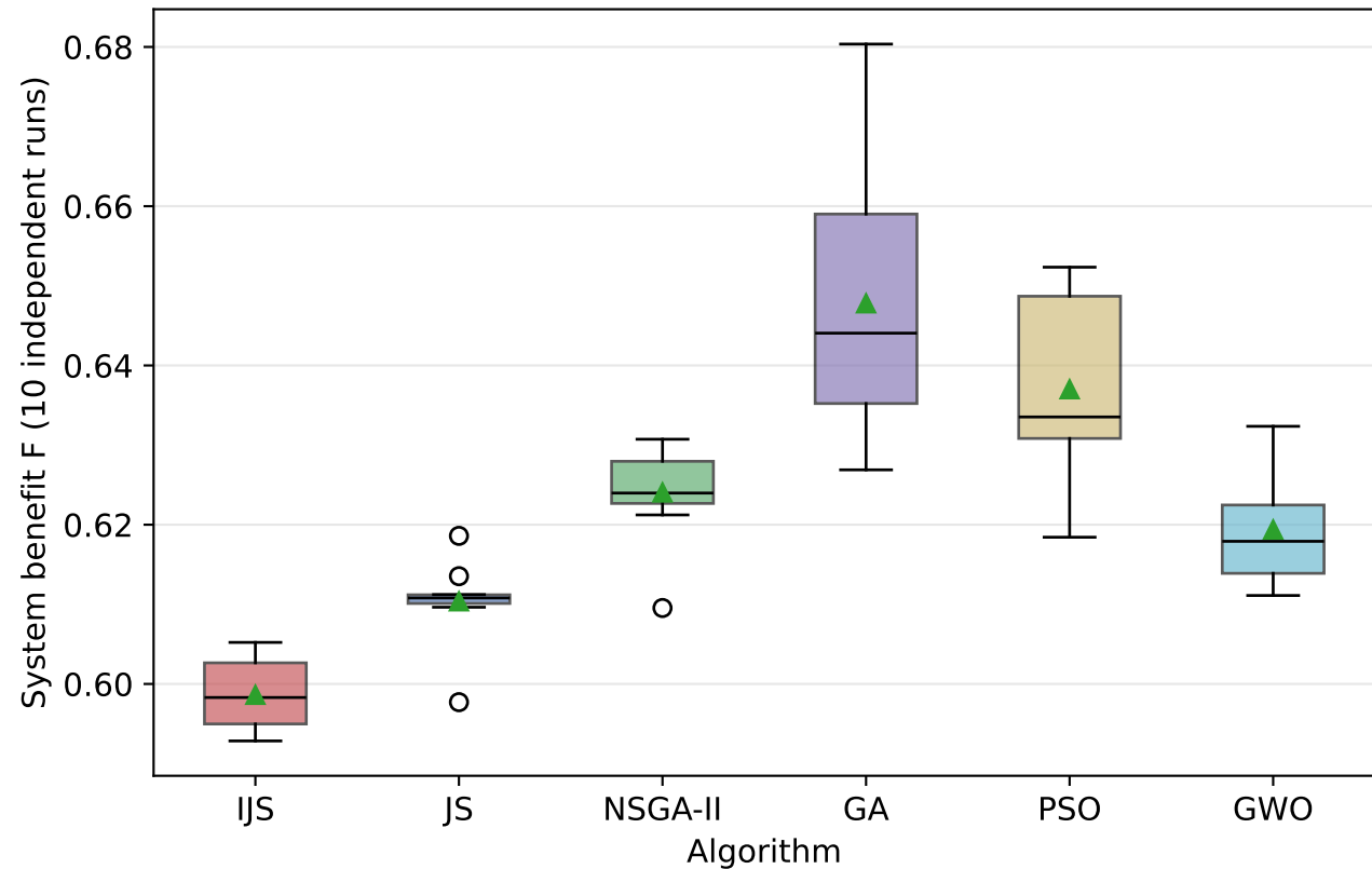
Fig. B4 Box plots of system benefit F across algorithms (scale PJ2 (400 m))
