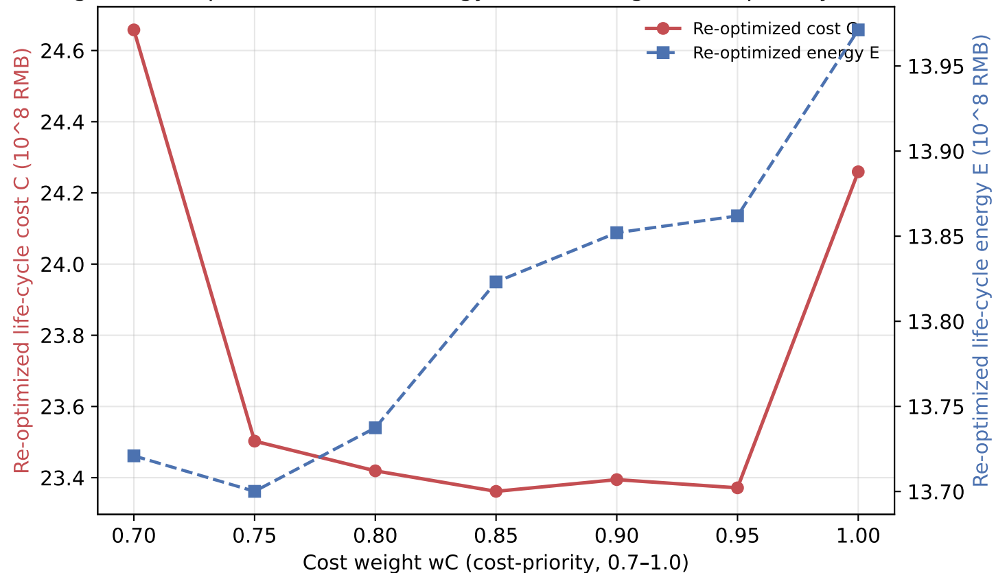
Fig. D6 Re-optimized cost & energy vs cost weight (cost-priority 0.7–1.0)
