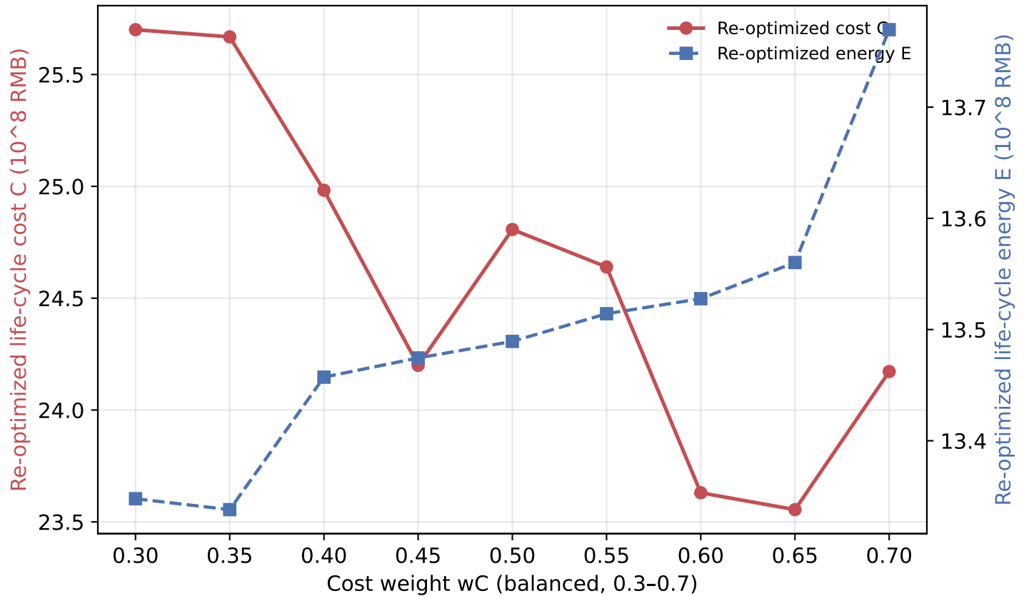
Fig. D8 Re-optimized cost & energy vs weight (balanced, wC & wE each 0.3–0.7)
