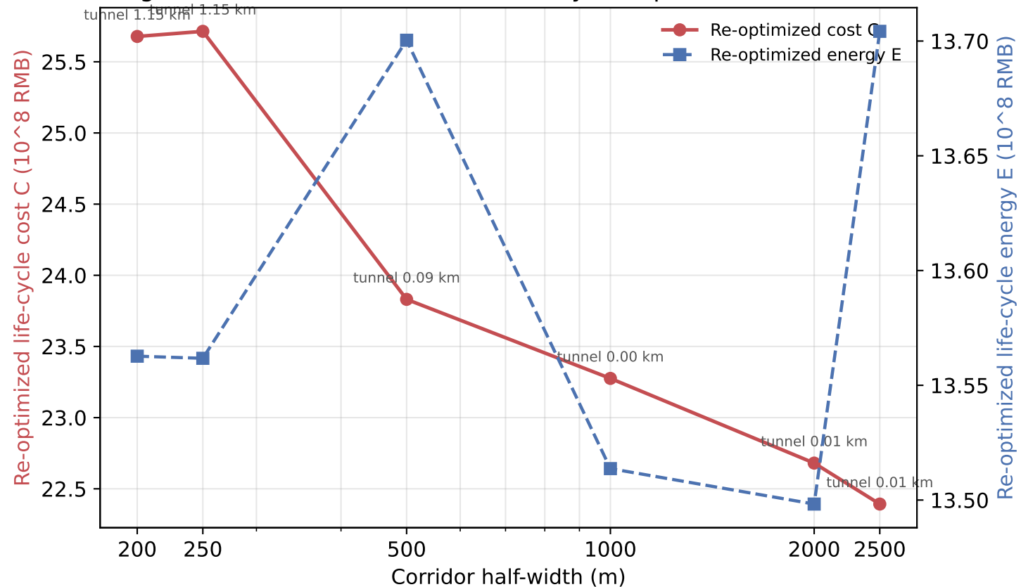
Fig. D9 Corridor half-width sensitivity (re-optimized, w1=0.65)
