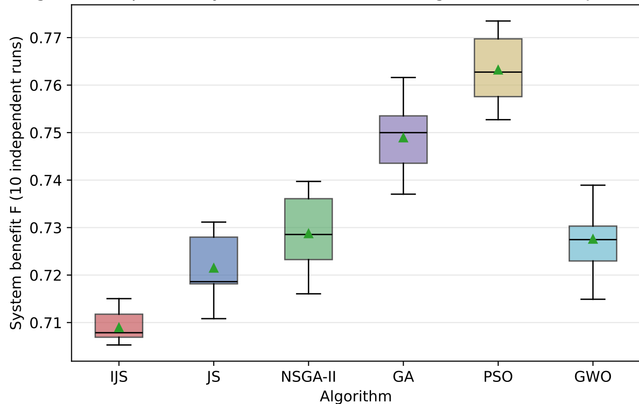
Fig. B4 Box plots of system benefit F across algorithms (scale PJ4 (200 m))
