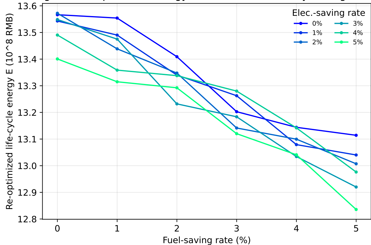
Fig. D3 Re-optimized energy vs fuel- and electricity-saving rates
