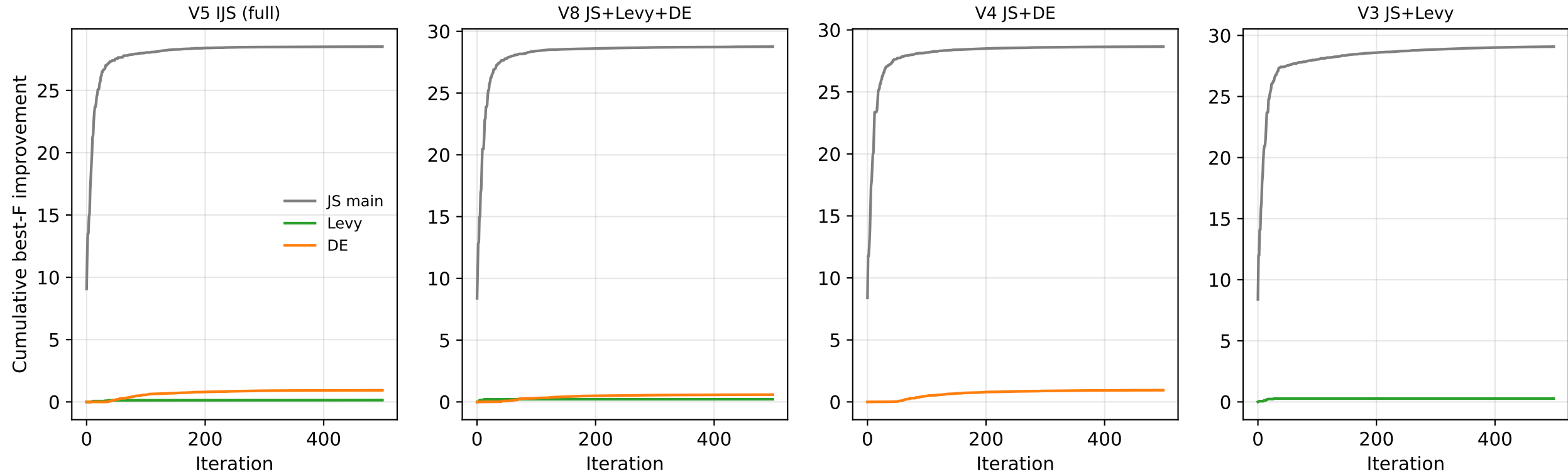
Fig. A4 Per-phase attribution of best-F improvement (tracked seed)
