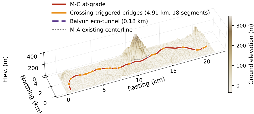
Fig. C11 Optimized alignment M-C on quasi-natural terrain (vertical exaggeration \approx 9\times )
