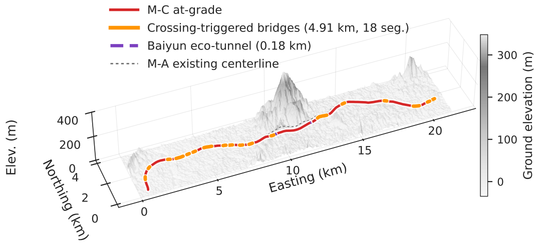
Fig. C11 (vB) Optimized alignment M-C on quasi-natural terrain (vert. exag. \approx 9\times )
