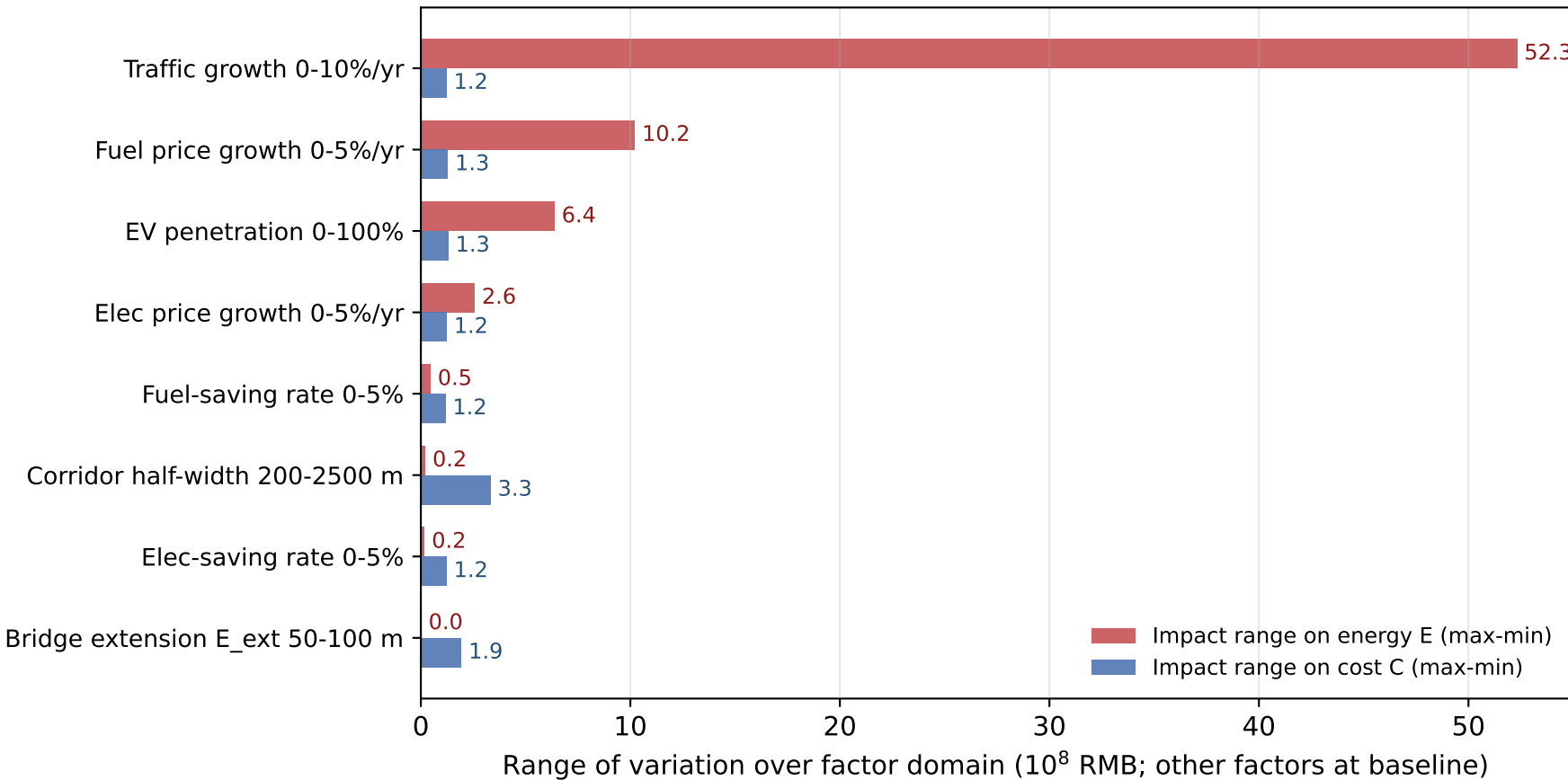
Fig. D11 Sensitivity tornado: traffic dominates E, cost C robust to all factors (every point fully re-optimized; items 1-3 sliced at baseline of the other factor)
