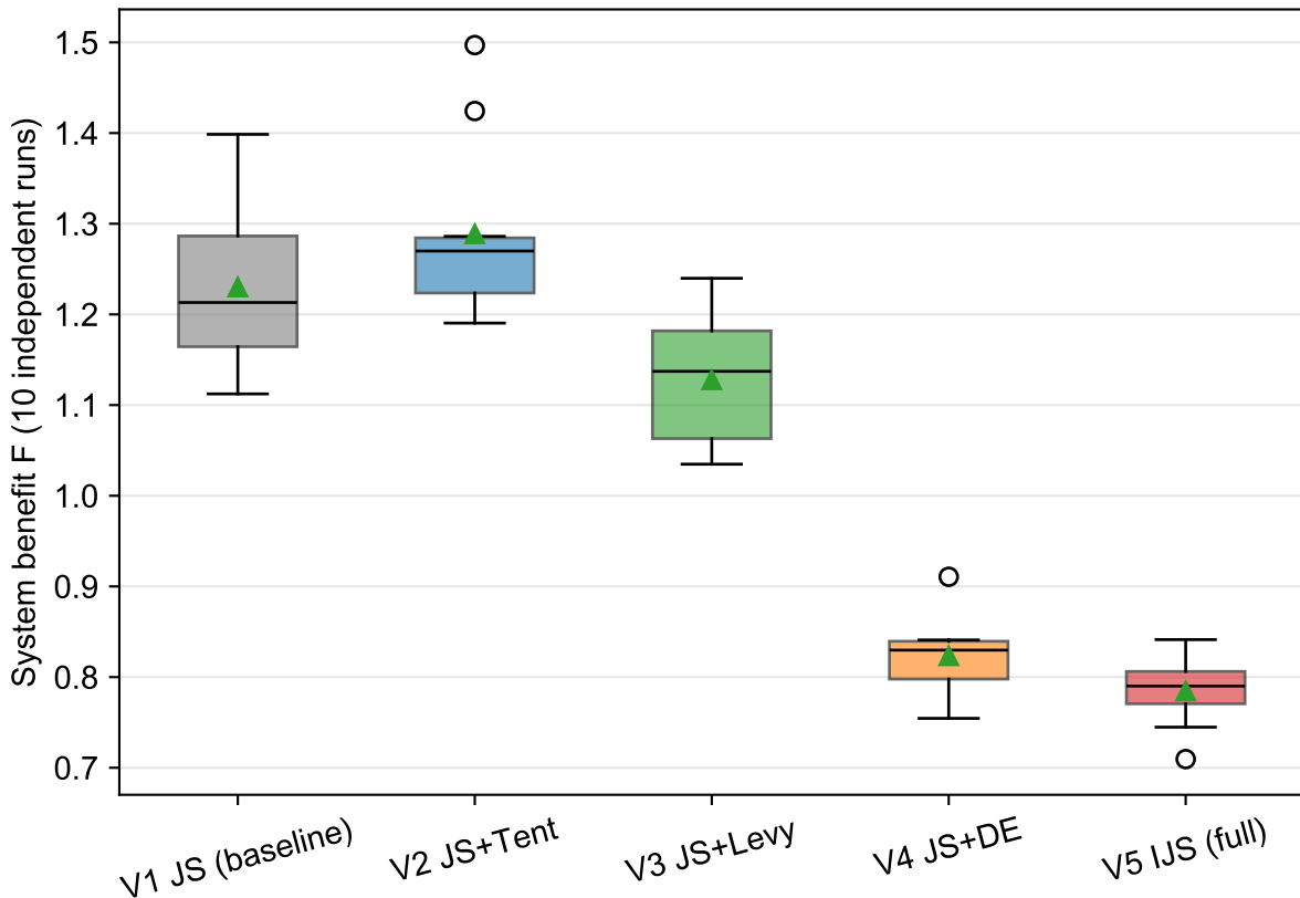
Fig. A3 Box plots of 10 independent runs for each ablation variant
