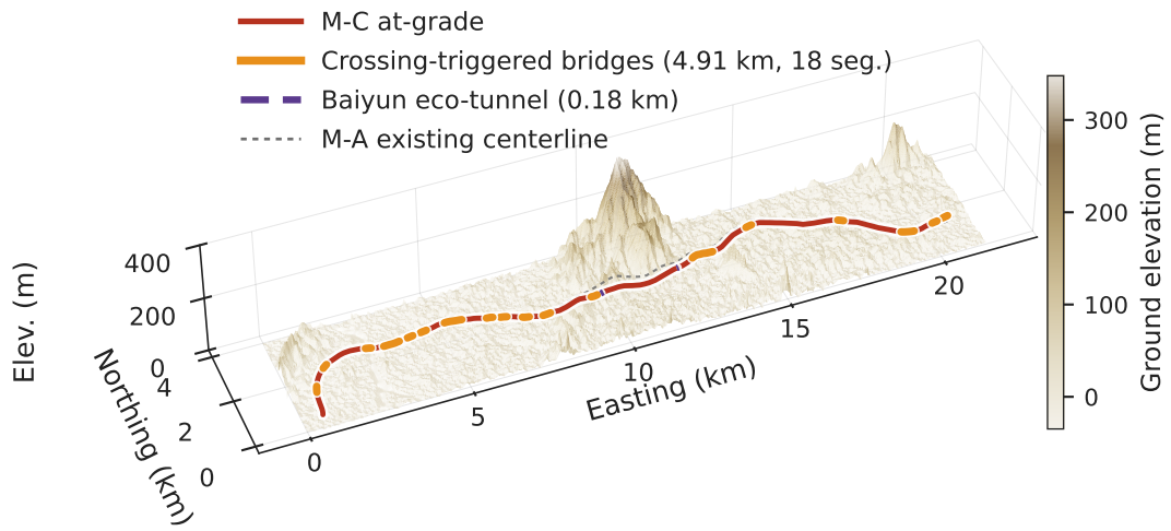
Fig. C11 (vA) Optimized alignment M-C on quasi-natural terrain (vert. exag. \approx 9\times )
