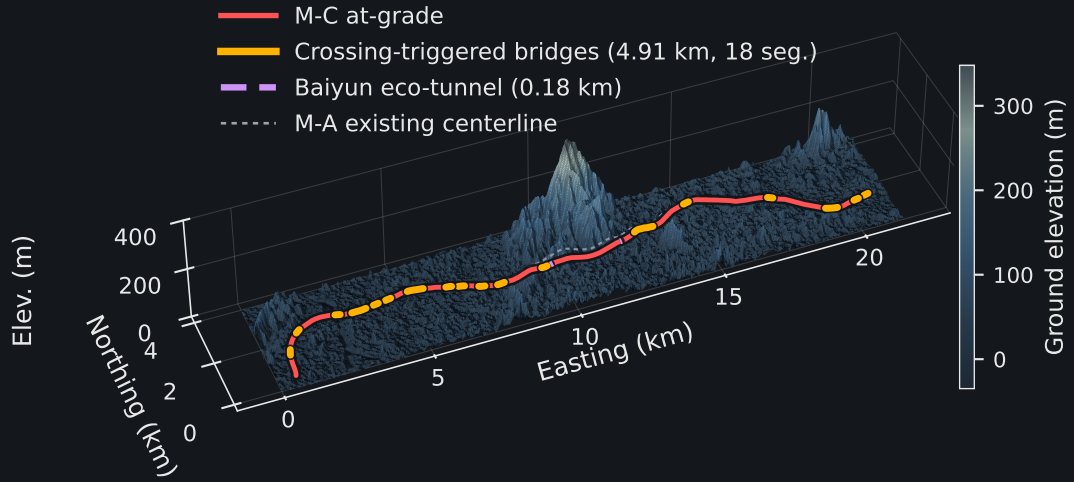
Fig. C11 (vD) Optimized alignment M-C on quasi-natural terrain (vert. exag. \approx 9\times )
