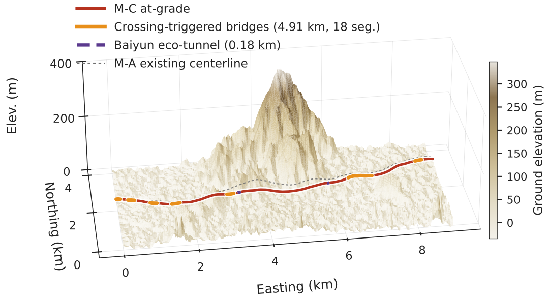
Fig. C11 (vE) Optimized alignment M-C on quasi-natural terrain (vert. exag. \approx 8\times )
