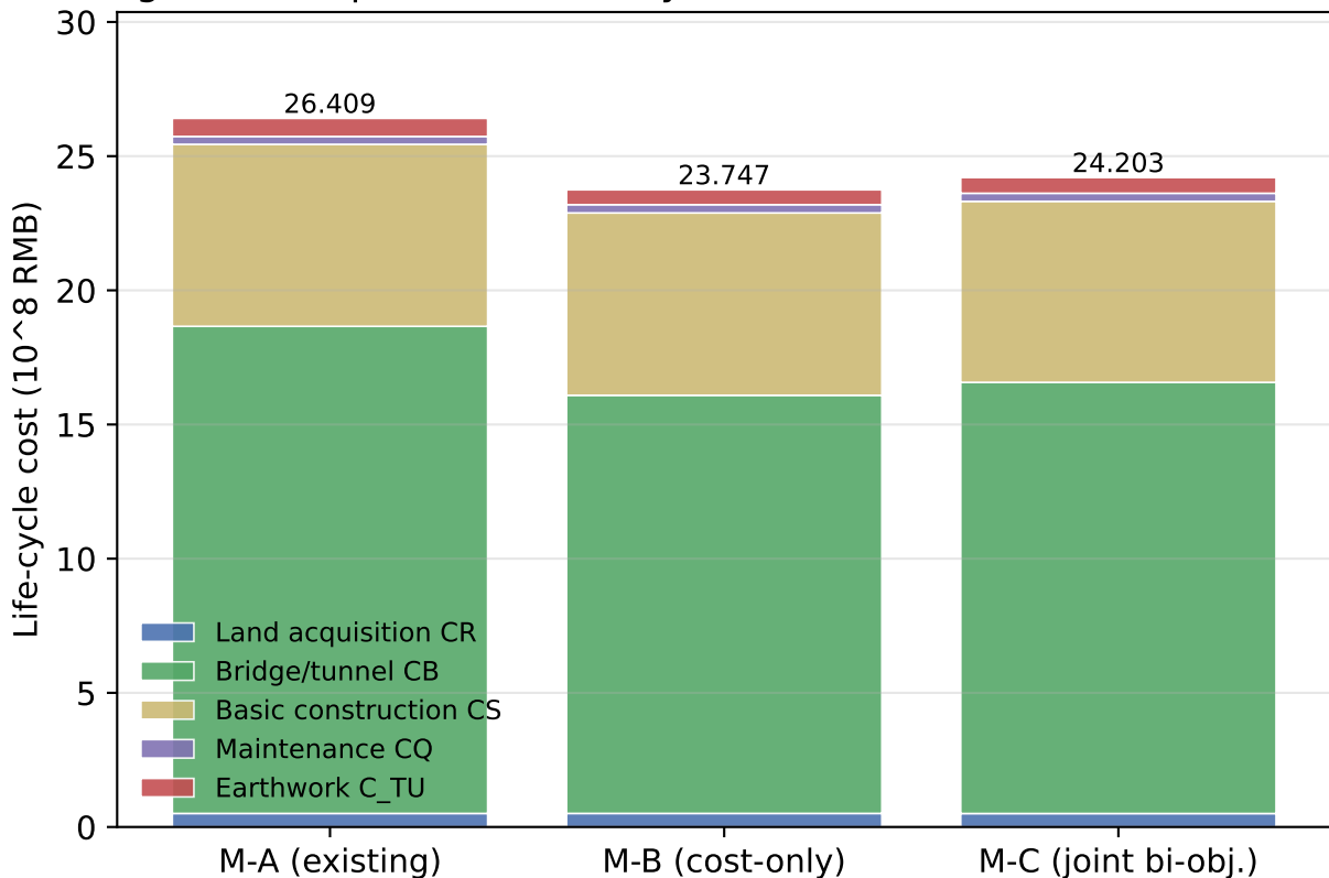
Fig. C4 Composition of life-cycle cost across the three schemes
