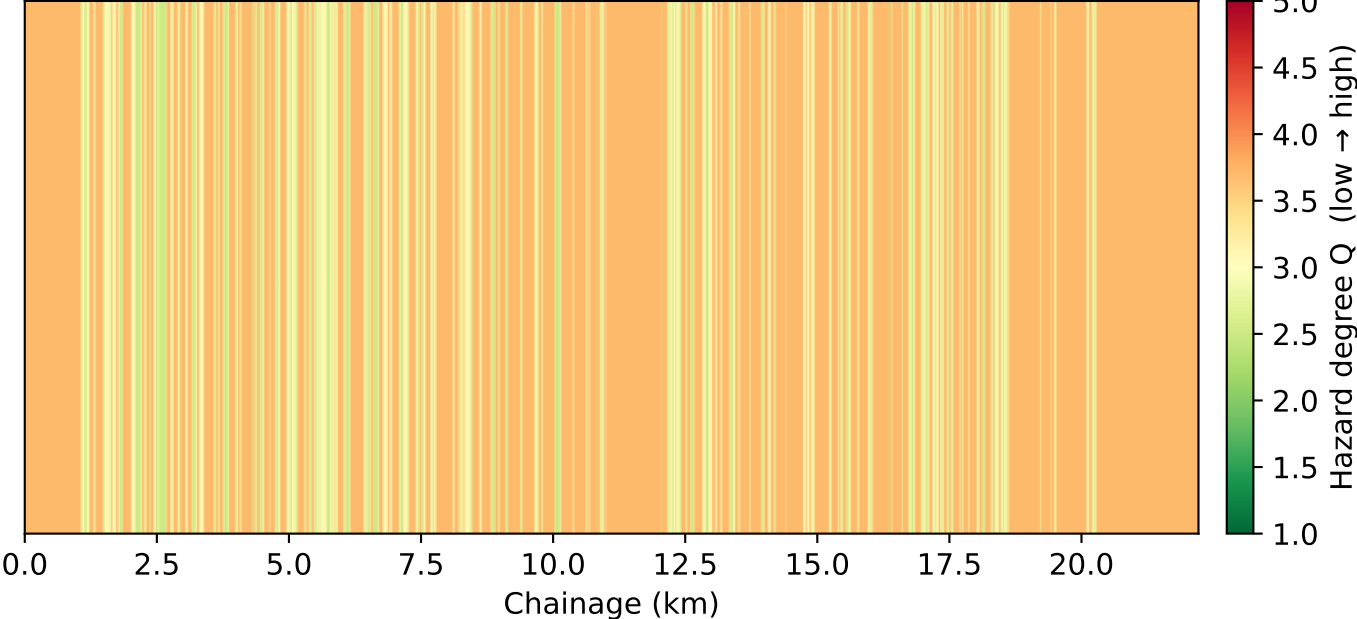
Fig. C5 Slope-stability hazard assessment of the optimized alignment (M-C)
