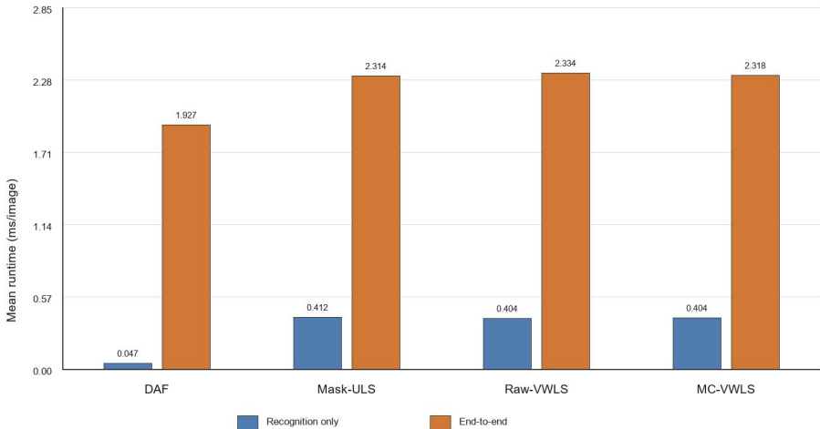
Single-image runtime of harmonic-recognition methods
