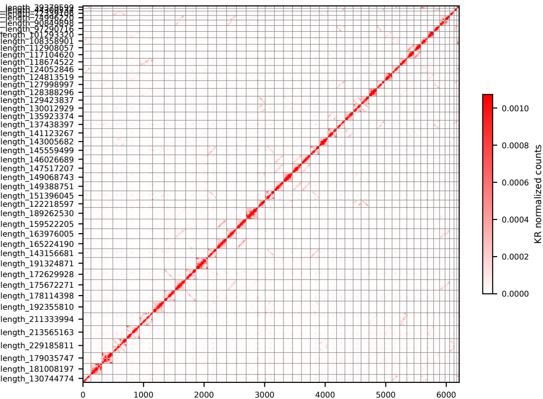
Hi-C contact map (bin size: 1000 Kb, x-axis unit: Mb)
