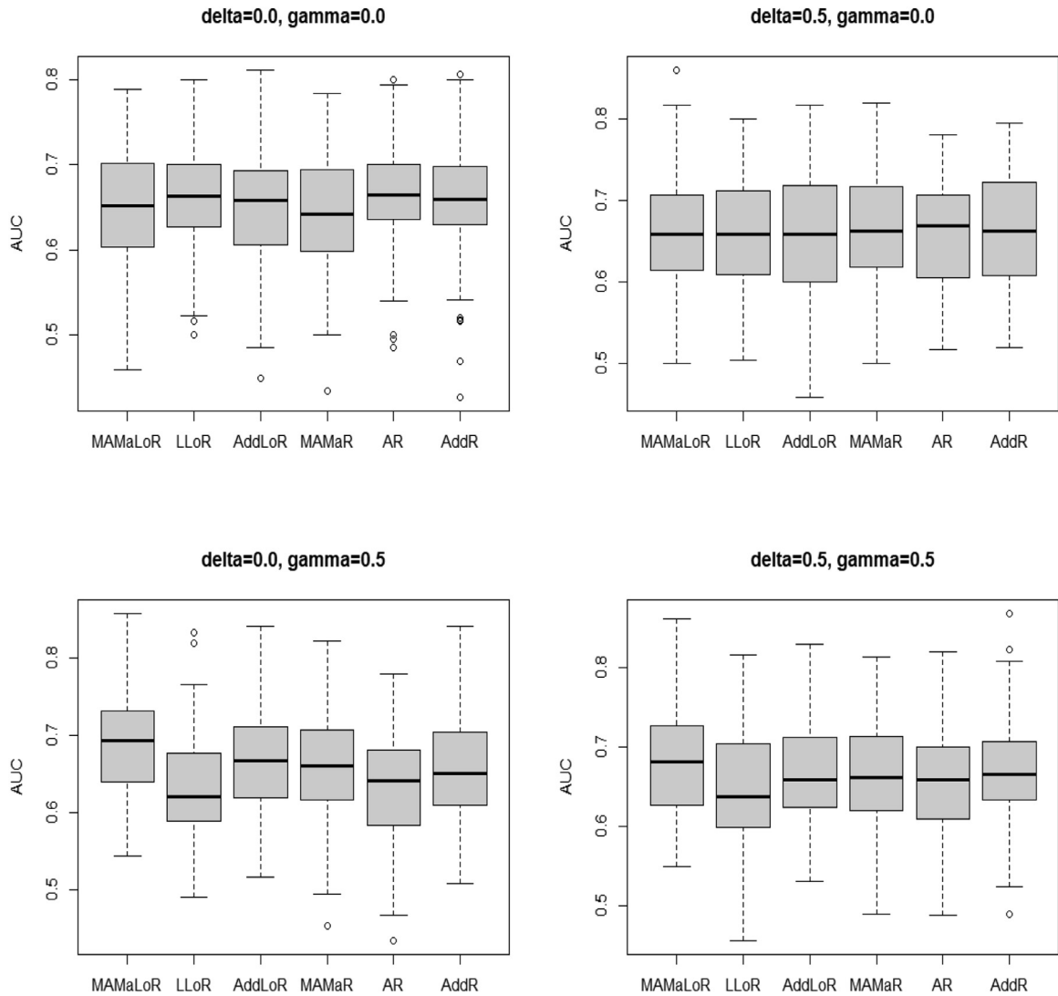
Fig. 2. Boxplots of the area under curve (AUC) with 100 repetitions for one-step ahead classification predictions, with n_p = 50 observations for testing, of different methods under different true model structures (Top left: linear, Top right: additive, Bottom left & right: nonlinear non-additive) based on n = 1000 observations for training.
