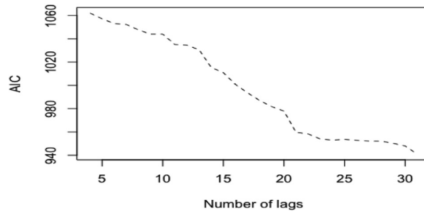
Fig. 7. The aic of MAMaLoR model with different number of lagged G_t .
