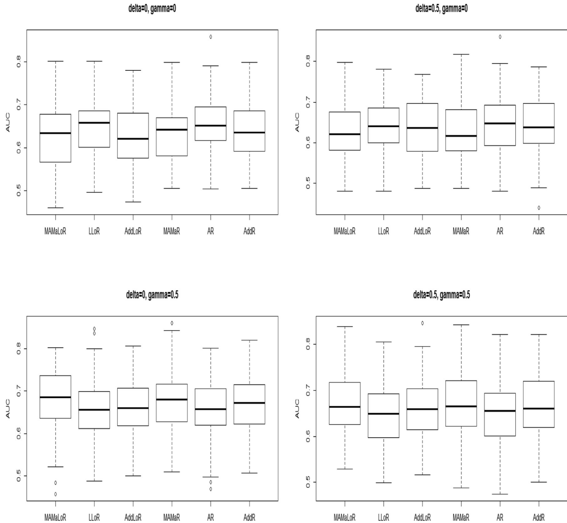
Fig. 1. Boxplots of the area under curve (AUC) with 100 repetitions for one-step ahead classification predictions, with n_p = 50 observations for testing, of different methods under different true model structures (Top left: linear, Top right: additive, Bottom left & right: nonlinear non-additive) based on n = 500 observations for training.
