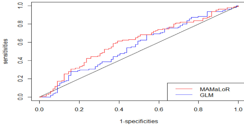
Fig. 8. The ROC curves for the MAMaLoR with selected bandwidth ( h given in Table 5) and the GLM models. Here the corresponding AUC values for MAMaLoR 0.6041 with h selected, and for GLM it is 0.560, respectively.
