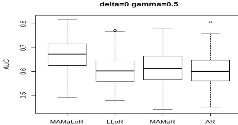
Fig. 3. Boxplots of the area under curve (AUC) with 100 repetitions for one-step ahead classification predictions of non-additive data, with n_p = 50 observations for testing, for \text{lag} = 31 , based on n = 1000 observations for training.
