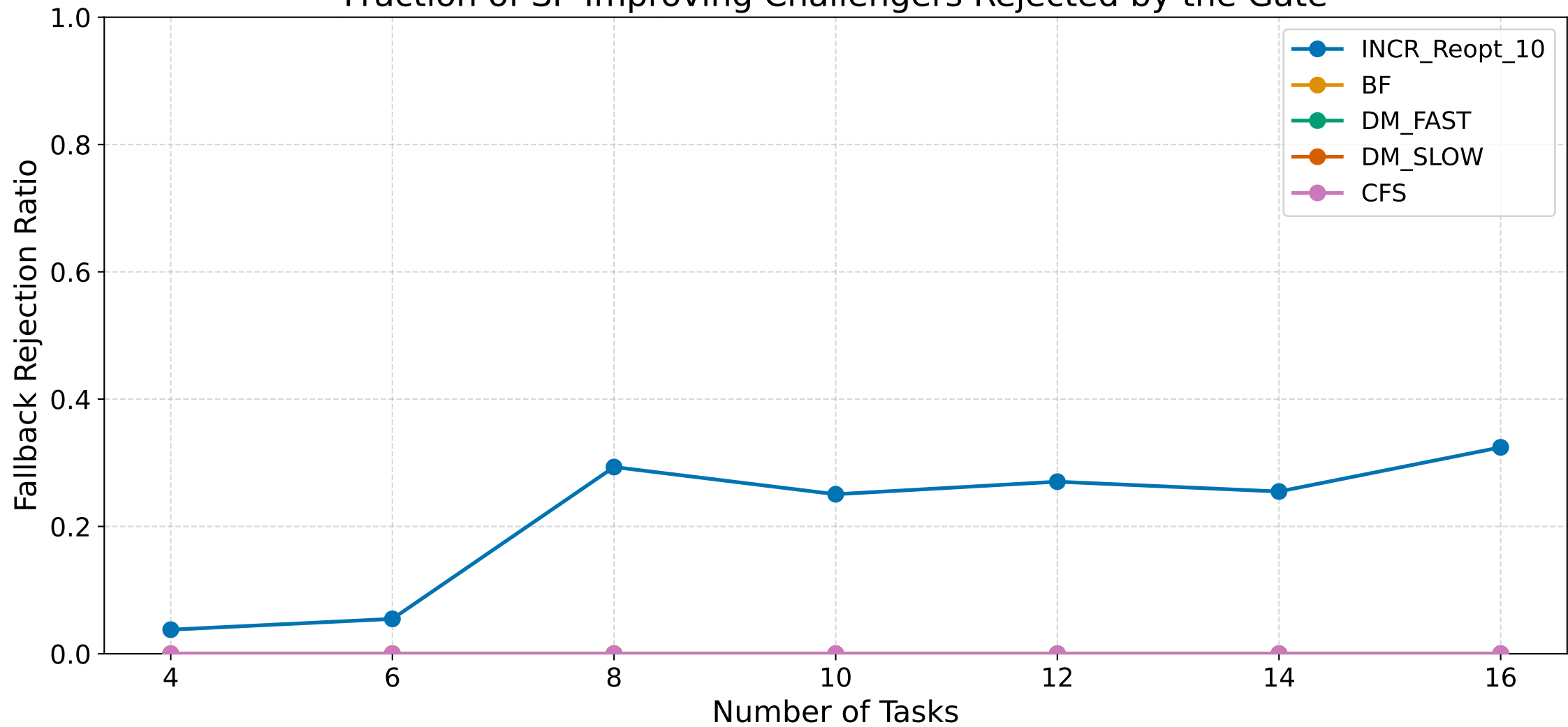
Fraction of SP-Improving Challengers Rejected by the Gate
