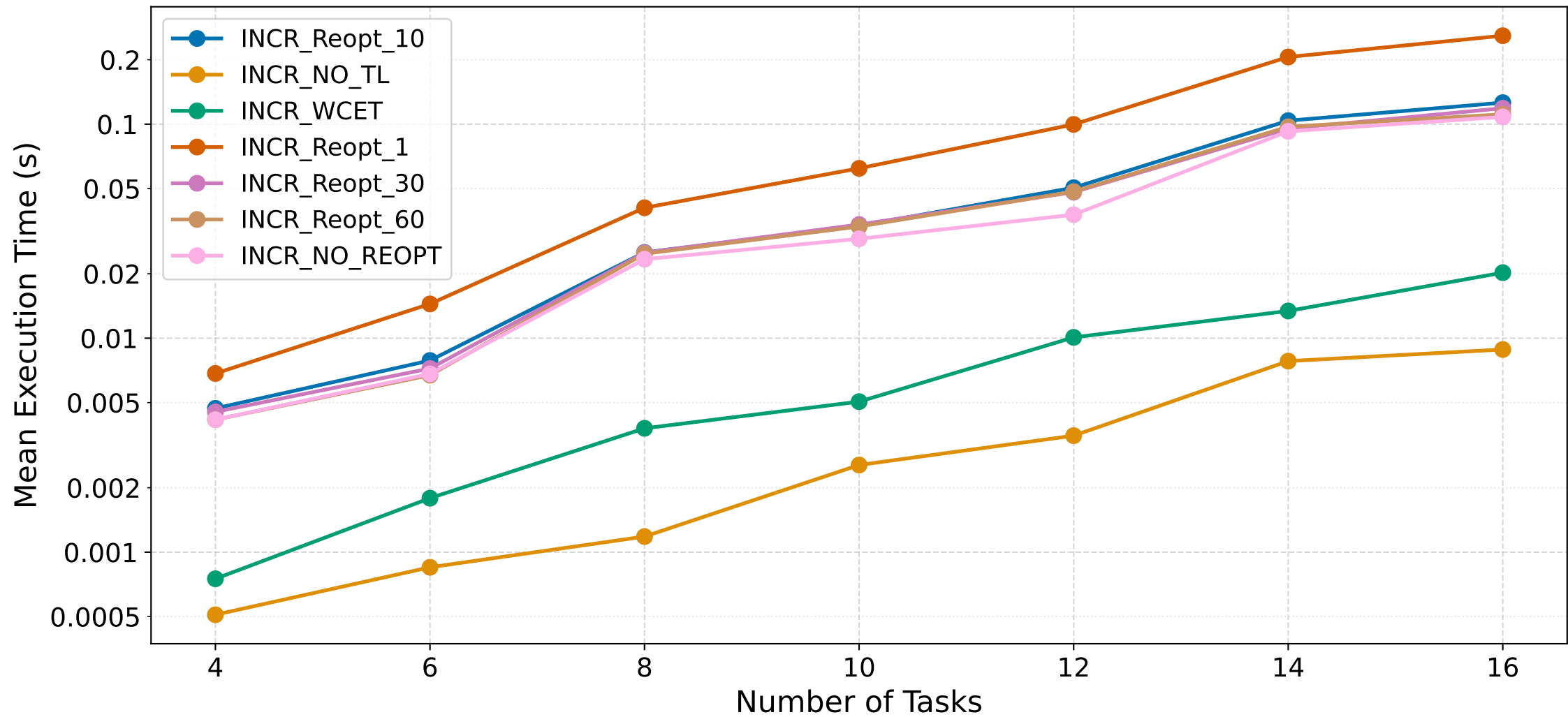
Mean Execution Time vs. Number of Tasks (Ablation)
