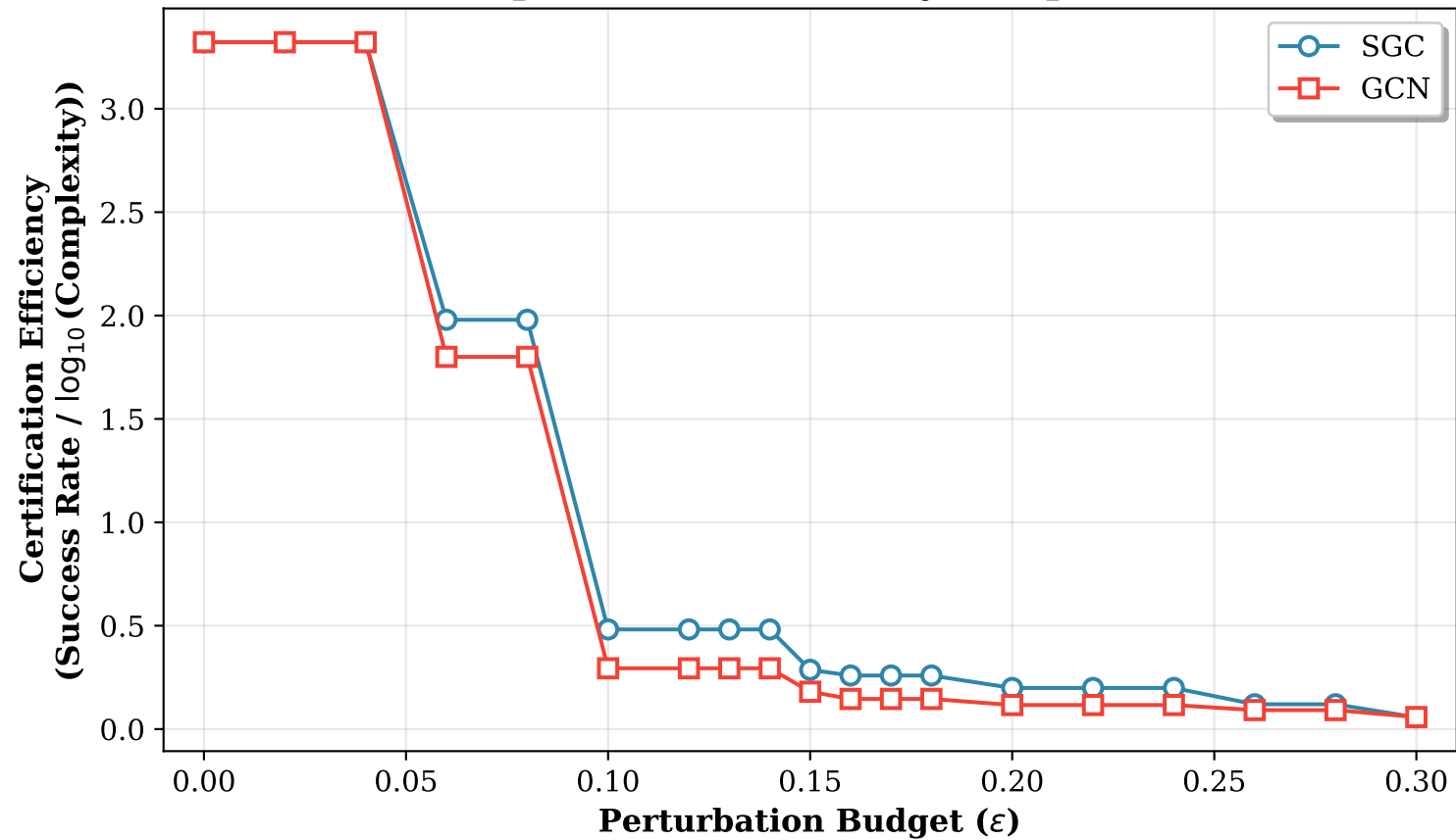
Computational Efficiency Comparison
