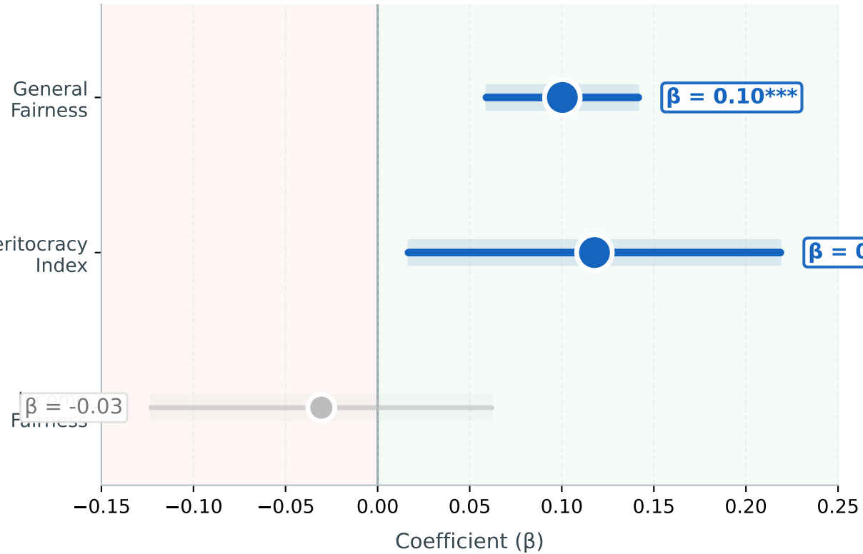
OLS Regression
