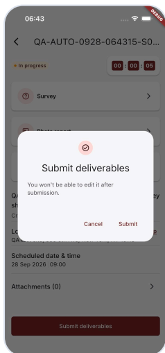
07 · Submit deliverables –
