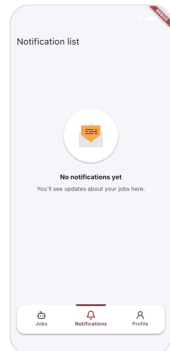
11 · Notifications – notifications-empty
