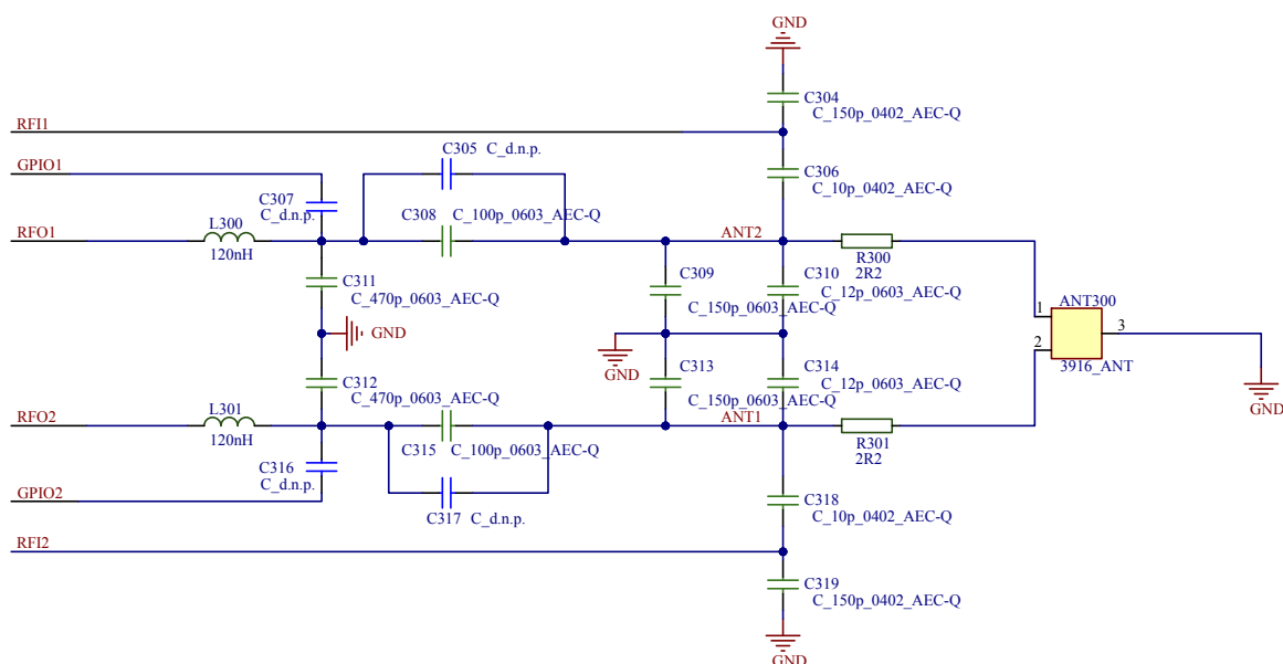
Figure 3. ST25R500 matching circuit minimum configuration
