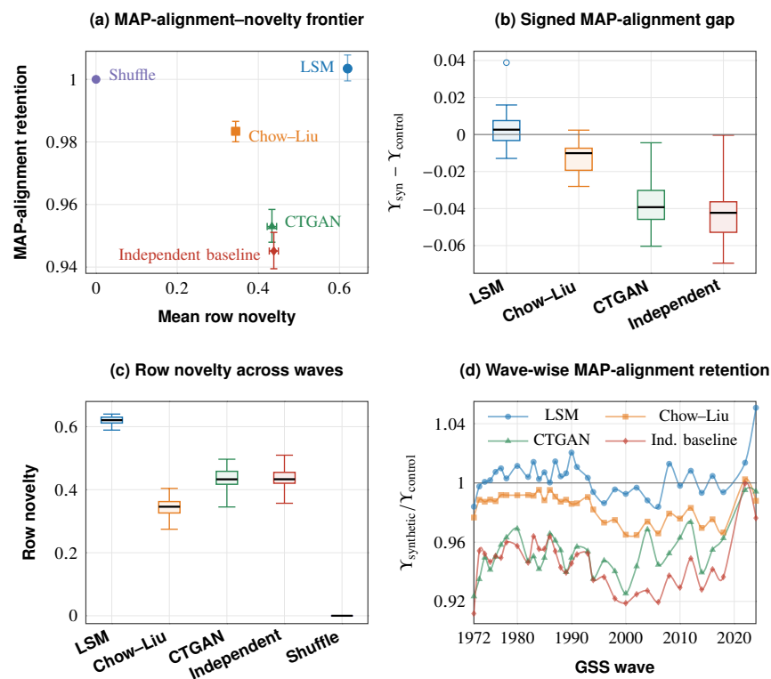
Fig. 1. Four complementary views of the GSS benchmark. (a) Cross-wave MAP-alignment–novelty frontier with nonparametric 95% wave-bootstrap intervals. (b) Wave-level signed MAP-alignment differences from the original-row control. (c) Wave-level row novelty, defined as one minus mean nearest-real similarity. (d) MAP-alignment retention by GSS wave. The label “Chow-Liu” denotes the restricted Chow-Liu hybrid.
