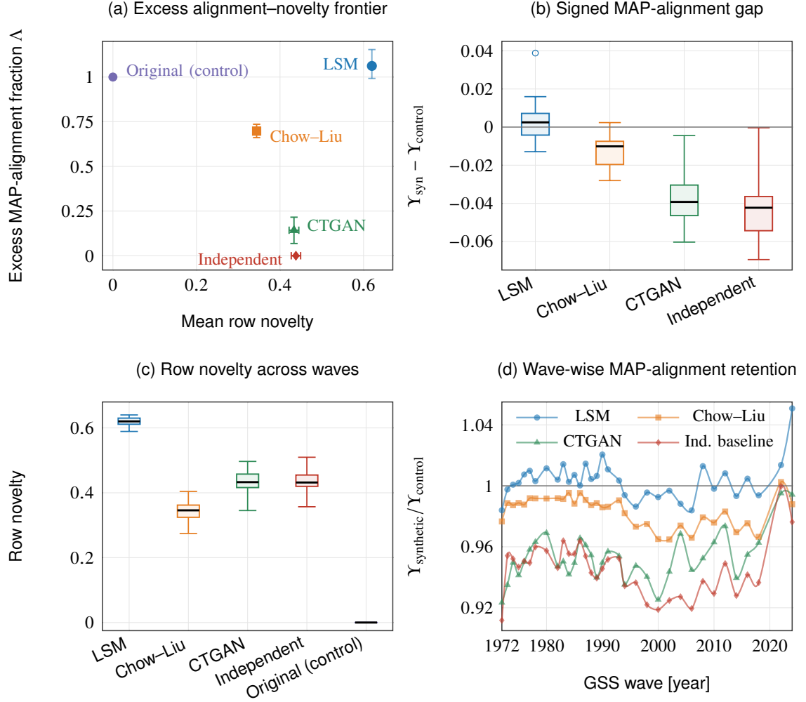
Fig. 1. Four complementary views of the GSS benchmark: (a) the excess MAP-alignment fraction \Delta_g = (\tilde{\gamma}_g - \tilde{\gamma}_{\text{ind}})/(\tilde{\gamma}_{\text{control}} - \tilde{\gamma}_{\text{ind}}) against mean row novelty, with nonparametric 95% wave-bootstrap intervals; the independent-marginal baseline is anchored at zero and the original (control) at one; (b) wave-level signed MAP-alignment differences from the original (control); (c) wave-level row novelty, defined as one minus mean nearest-real similarity; and (d) MAP-alignment retention by GSS wave. The label “Chow-Liu” denotes the restricted Chow-Liu hybrid.
