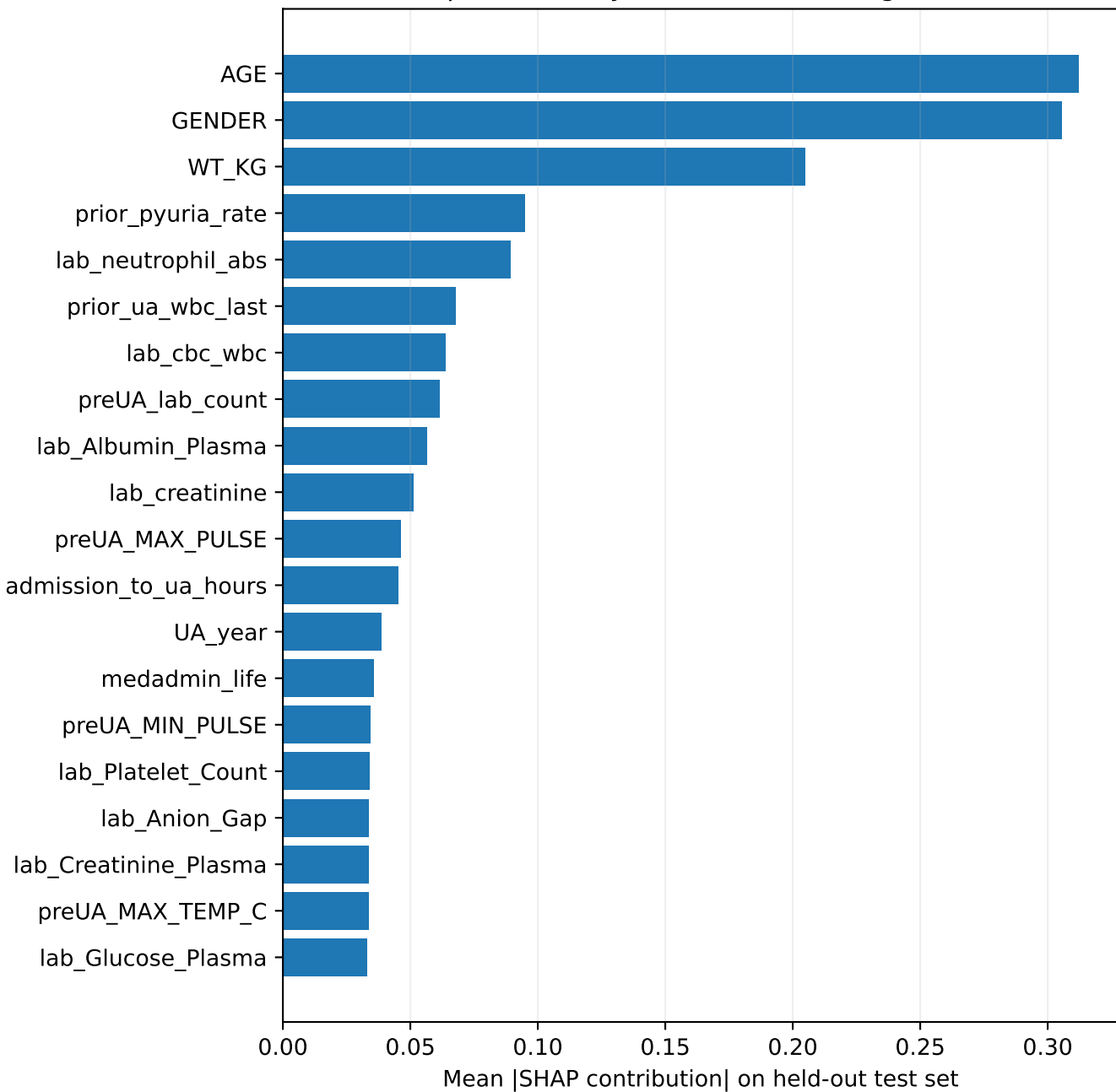
Top features by held-out SHAP magnitude
