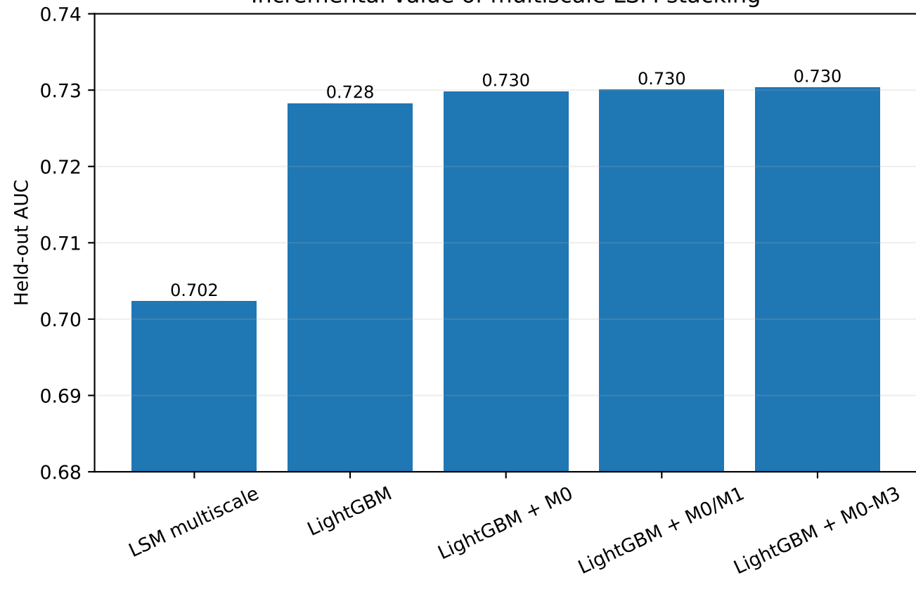
Incremental value of multiscale LSM stacking
