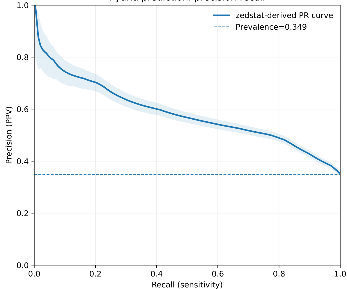
Pyuria prediction: precision-recall
