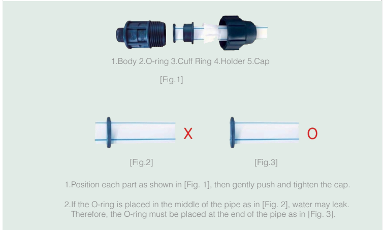
PE Compression Fitting Installation Method
