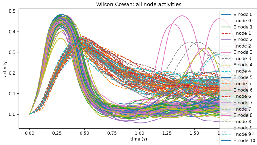
Figure 1: Simulation of the Wilson–Cowan model across 80 brain regions using Neurolib 2. The figure illustrates the spatiotemporal dynamics of excitatory and inhibitory populations, demonstrating inter-regional interactions mediated by structural connectivity and conduction delays. Stochastic fluctuations are introduced via Ornstein–Uhlenbeck noise, highlighting variability around deterministic trajectories.
