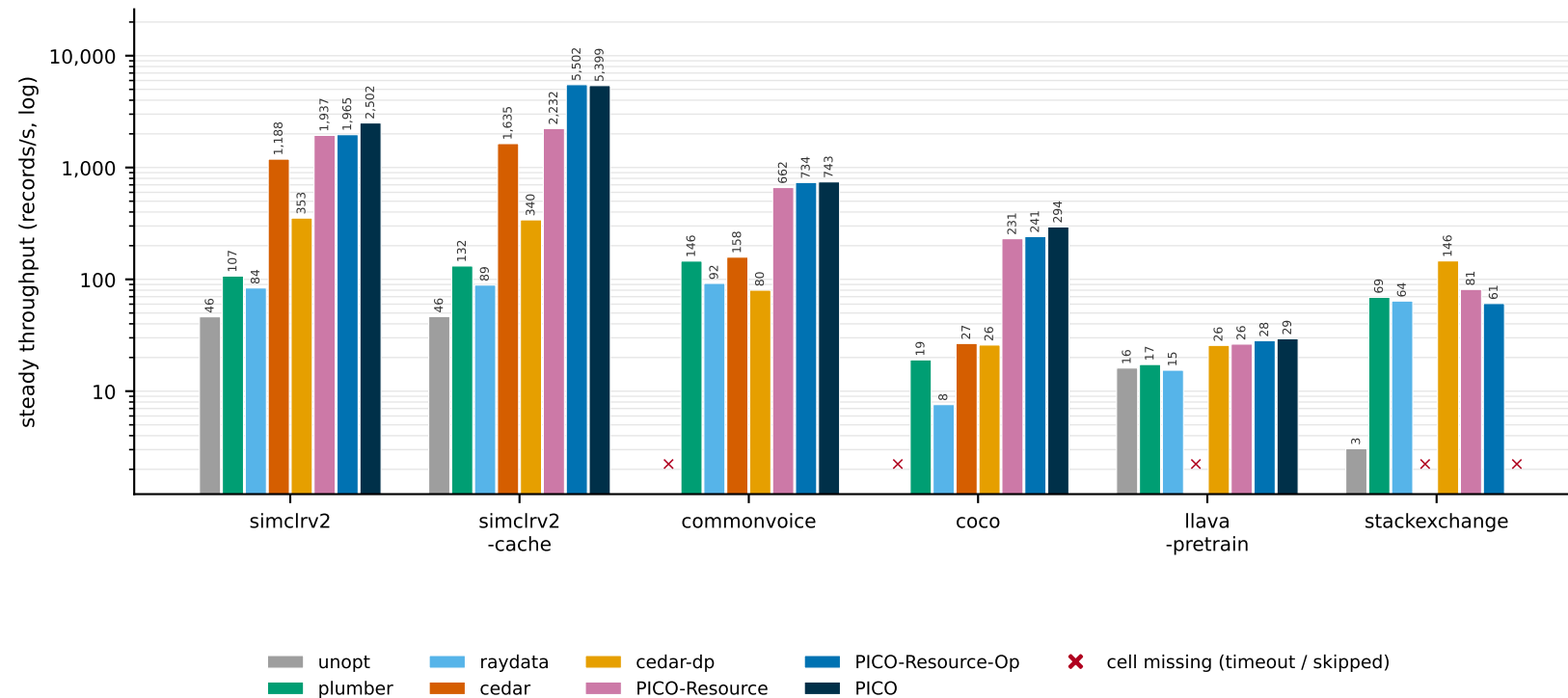
Steady-state throughput on the formal campaign (log scale)
