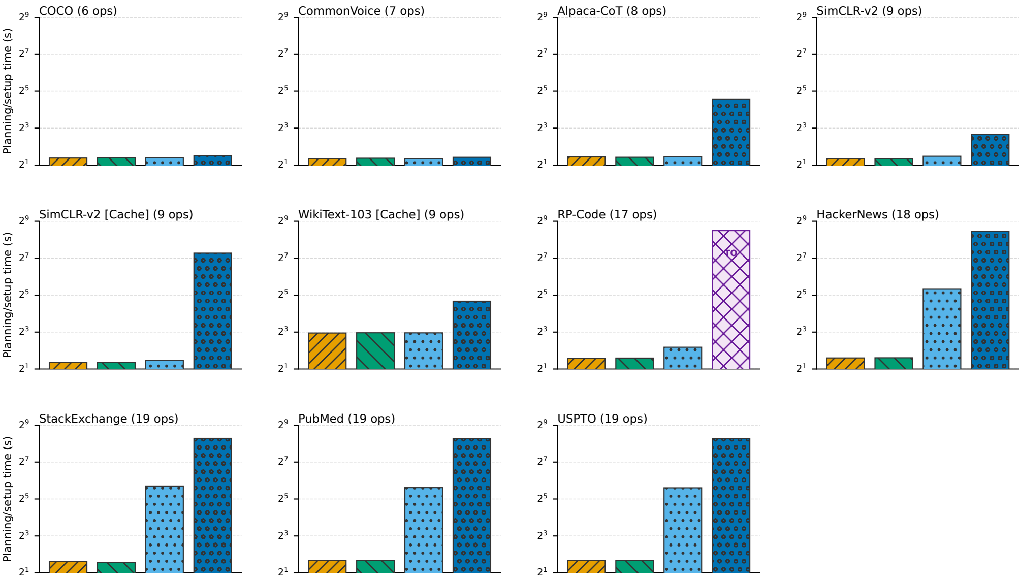
Planning and setup time (lower is better; \log_2 scale)
