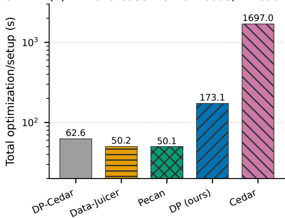
(b) 14 valid-baseline workloads; timeouts capped
