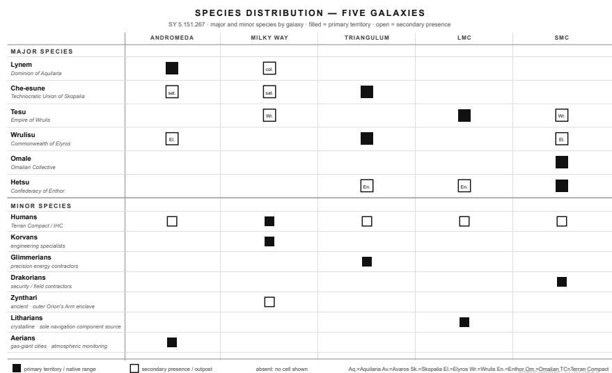
Figure 8: Species distribution across the Five Galaxies
