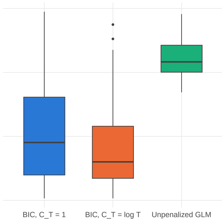
Zero-inflated data ( \pi_0 = 0.2 )
