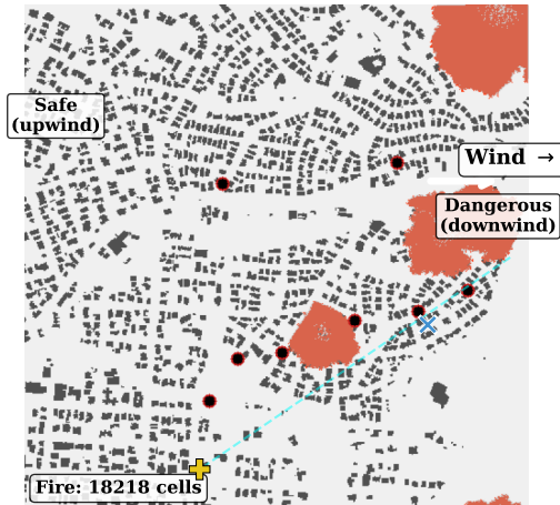
(b) Wind-driven fire (3 m/s W→E), t=150
