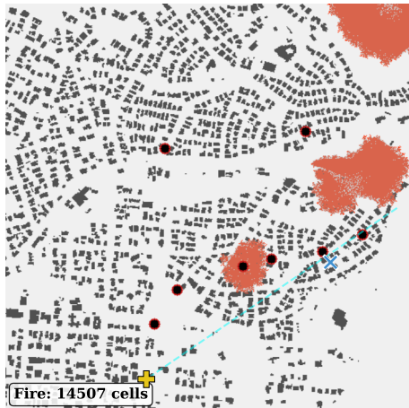
(a) Isotropic fire (no wind), t=150
