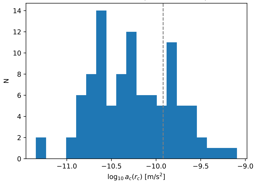
scatter = 0.44 dex (criterion: <0.3 )
