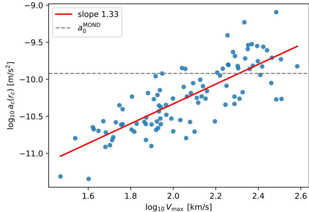
Characteristic acceleration at r_c vs V_{max}
