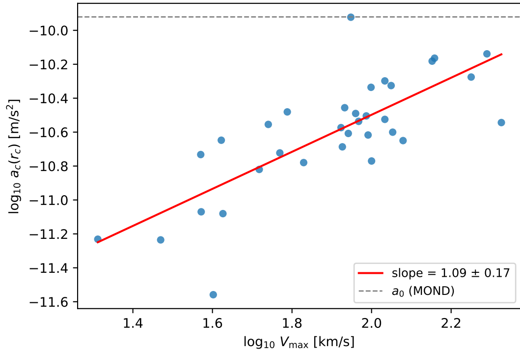
Fiducial run: a_c tracks V_{\max} ( \rho = 0.72 , n = 33 )
