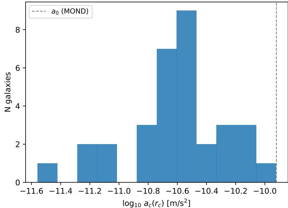
scatter = 0.34 dex (criterion: < 0.3 dex)
