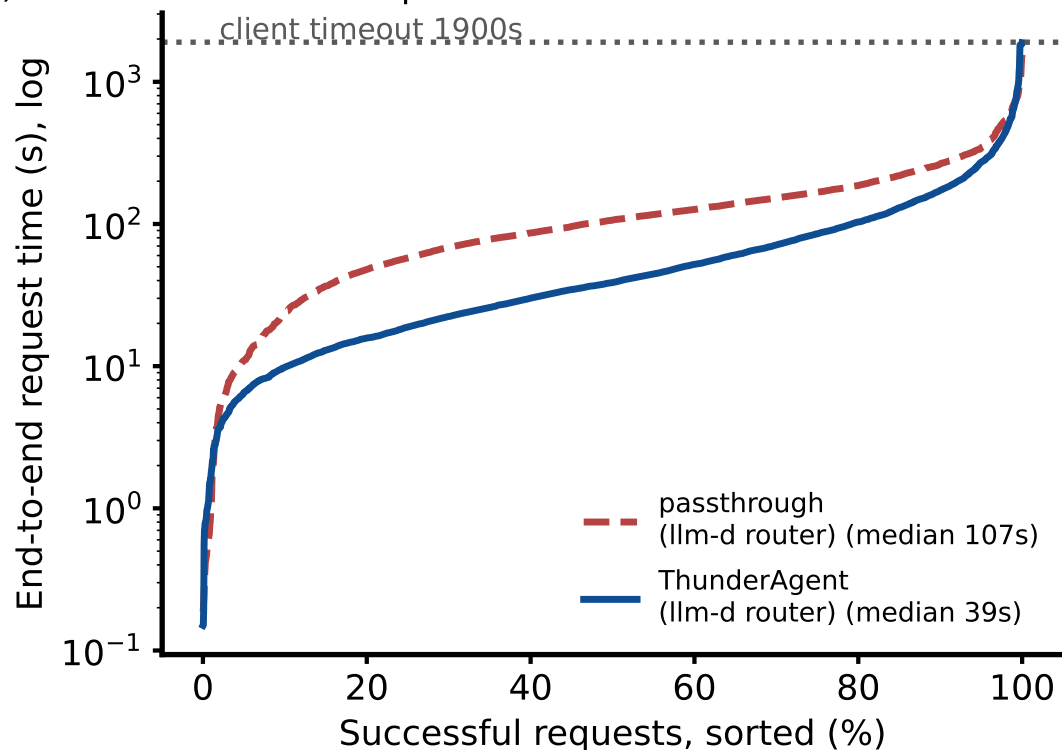
(b) Median successful request is 2.7x faster under the llm-d ThunderAgent
