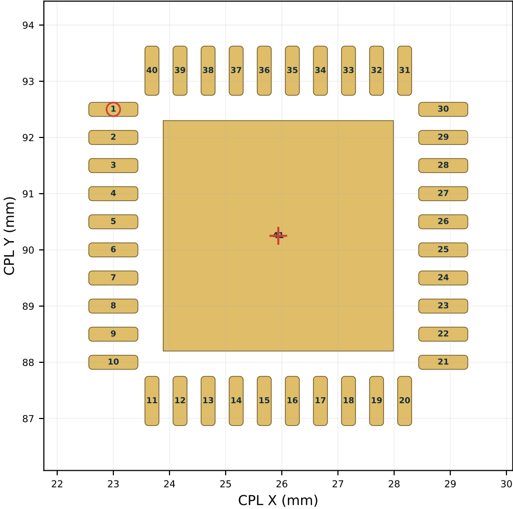
U6 | anchor (25.9375, 90.2500) mm | 0° top
