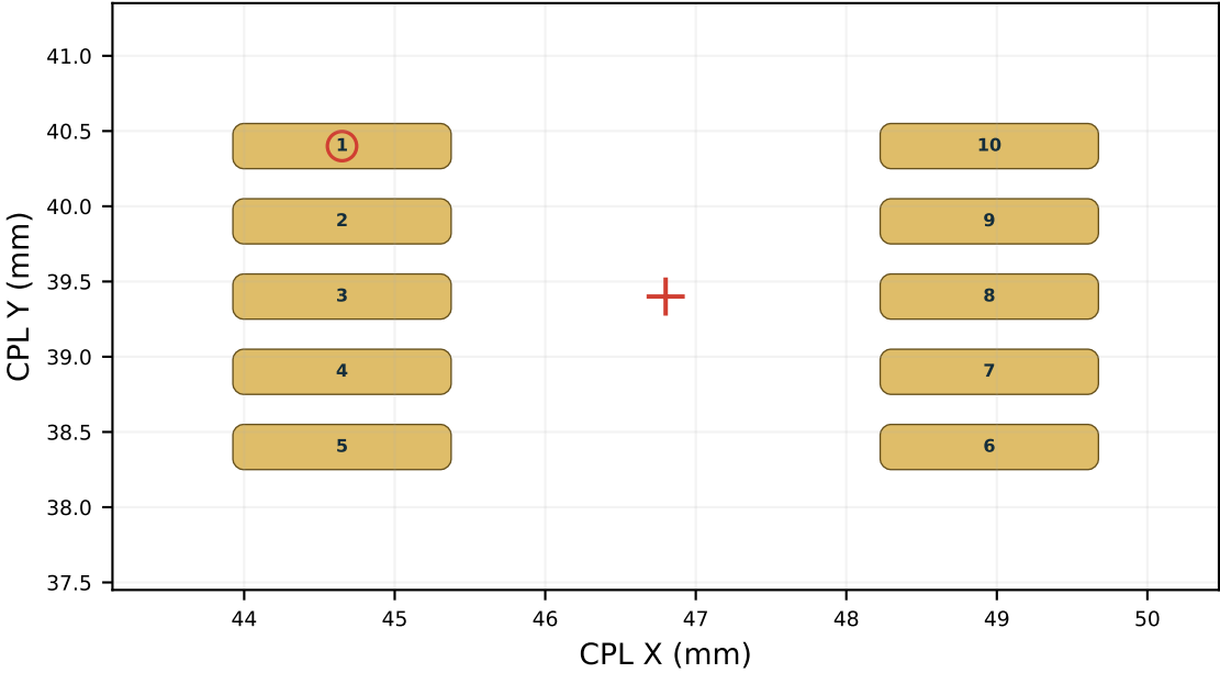
U10 | anchor (46.8000, 39.4000) mm | 0° top
