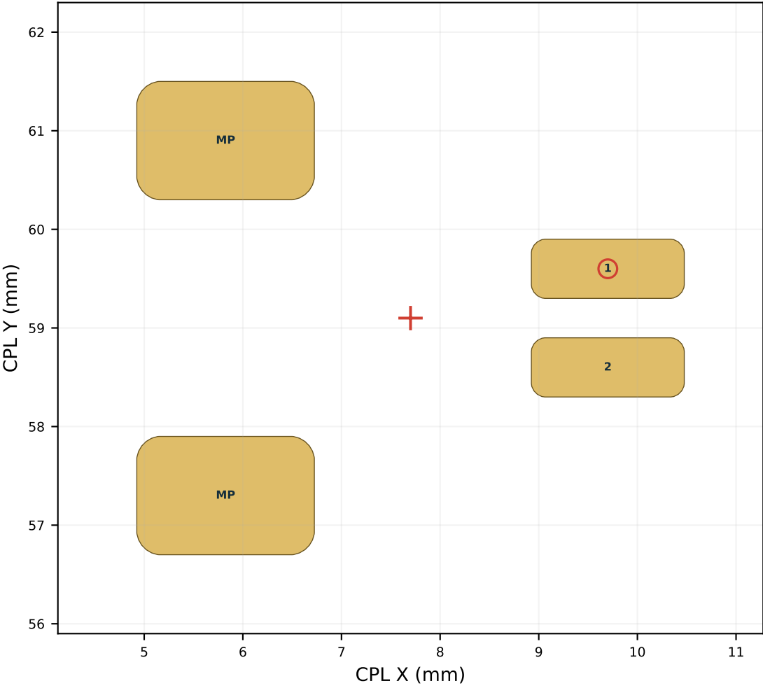
J2 | anchor (7.7000, 59.1000) mm | 270° top
