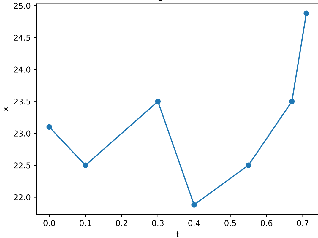
Signal x vs t
