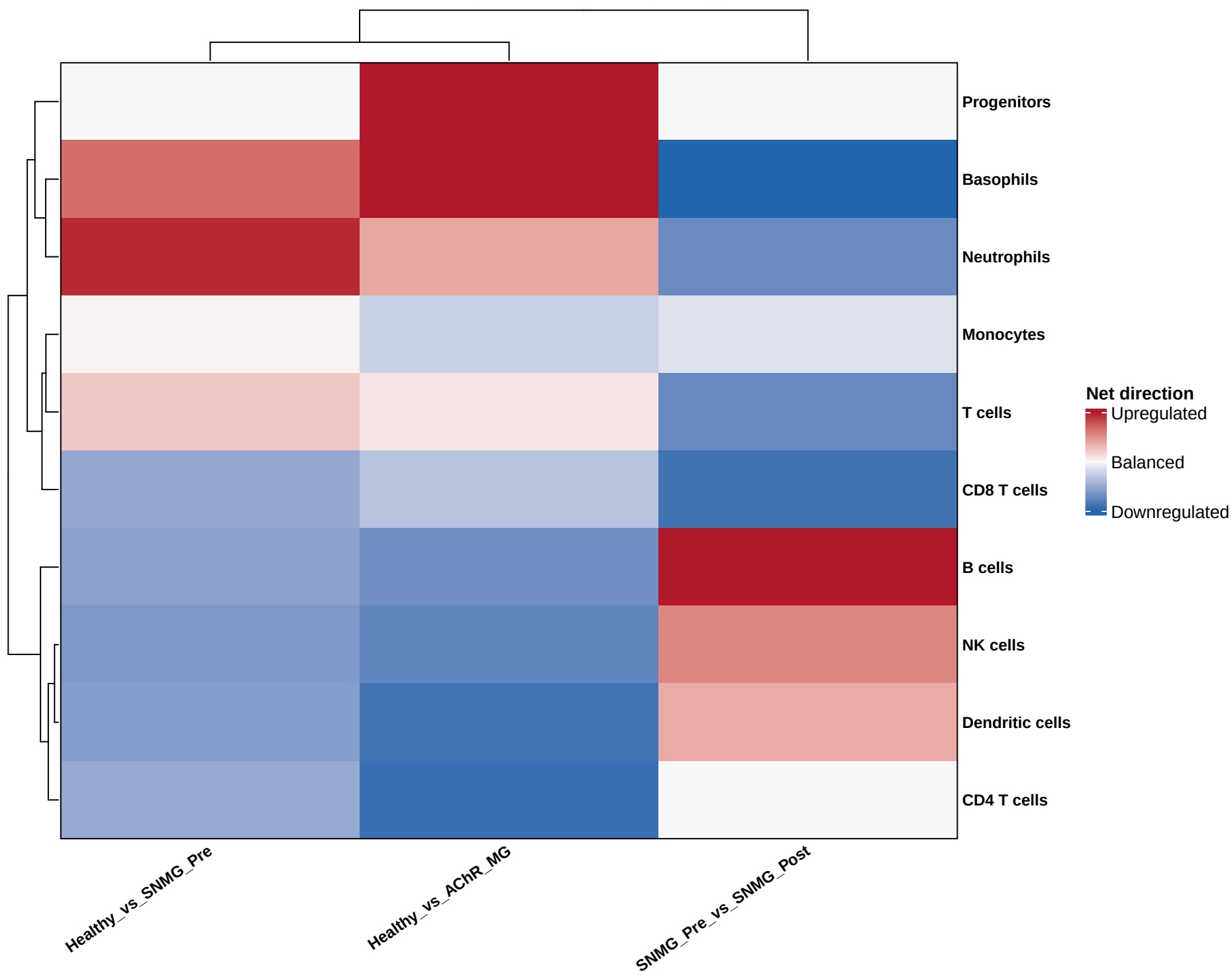
MG-associated transcriptional direction by comparison
